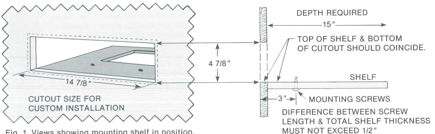
Fig. 1. Views showing mounting shelf in position.
