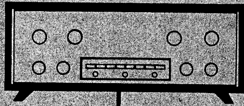
PROGRAM SOURCE
